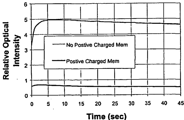
400mg/dl Glucose Test on Diff Membrane, Using Water Soluble Tetrazolium As Indicator
